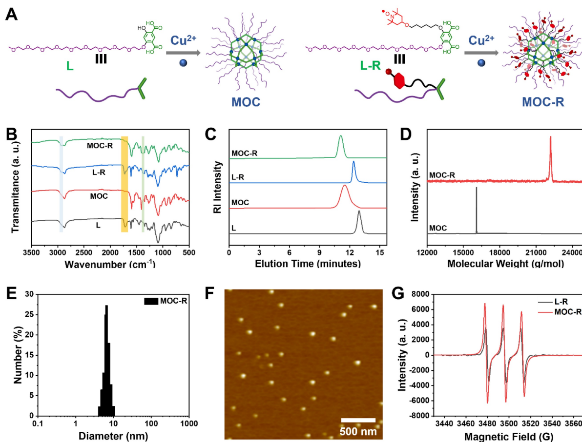
Figure 1. Preparation and Characterization of MOC-R cascade nanozyme. (A) The structures of ligands, MOC, and MOC-R. (B) The FT-IR spectra of ligands, MOC, and MOC-R. (C) The SEC profiles of the ligands, MOC, and MOC-R in THF. (D) The MALDI-TOF mass spectra of MOC and MOC-R. (E) The DLS plot of MOC-R in PBS. (F) The AFM image of MOC-R. Scale bars represent 500 nm. (G) The EPR curves of L-R and MOC-R.
